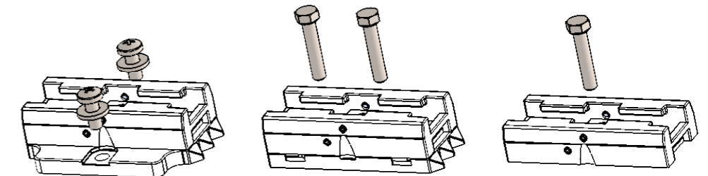
Slide bracket (wide)
